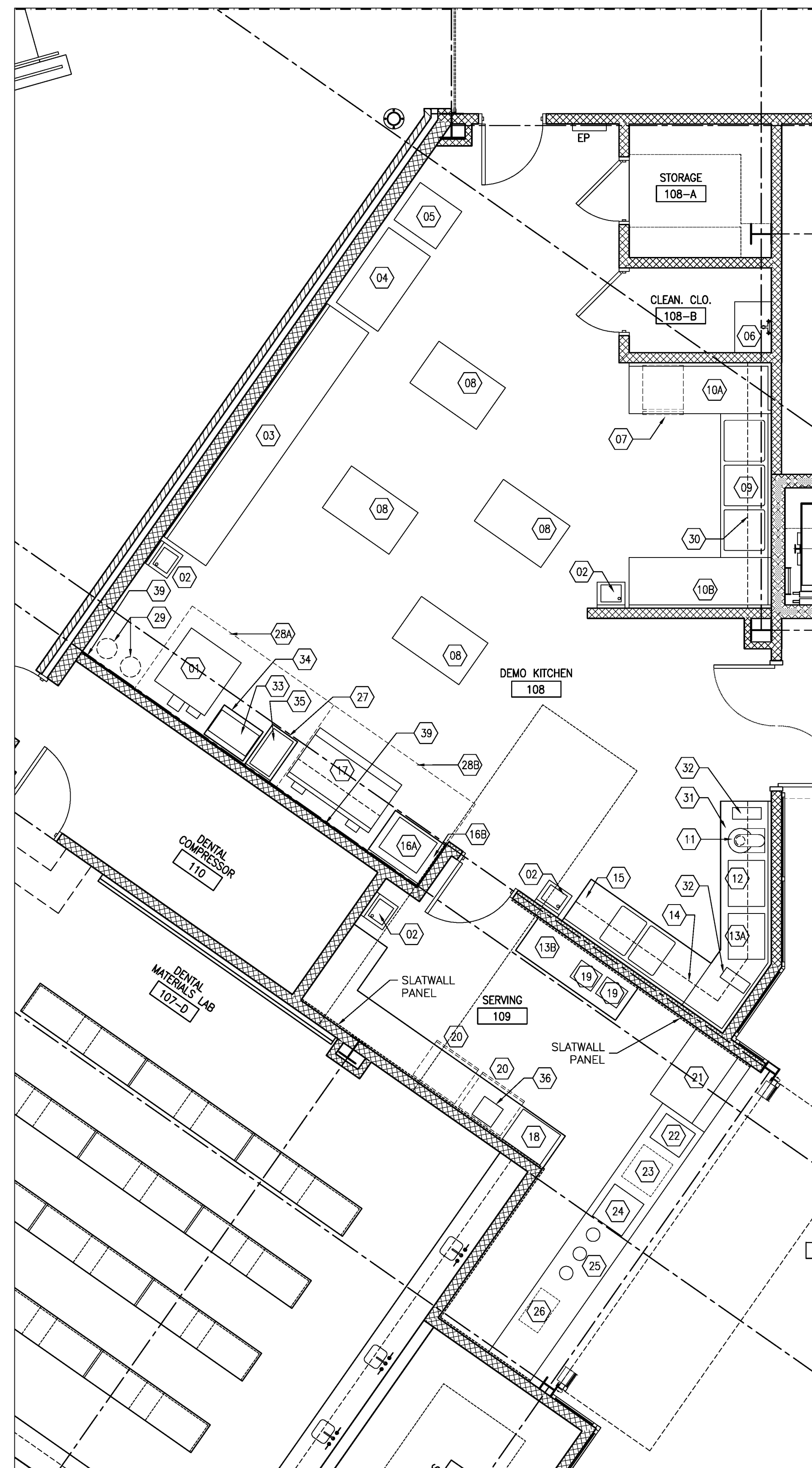
1 ENLARGED KITCHEN PLAN SCALE: 1/4" = 1'-0"
